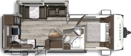
257RKS - Length: 29' 11" Weight: 5,562 lbs Fresh Water: 44 gals. Grey Water: 78 gals. Waste Water: 28 gals.
