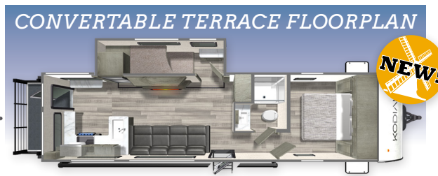
308BHS - Length: 34' 11" Weight: 6,635 lbs Fresh Water: 44 gals. Grey Water: 78 gals. Waste Water: 28 gals.
